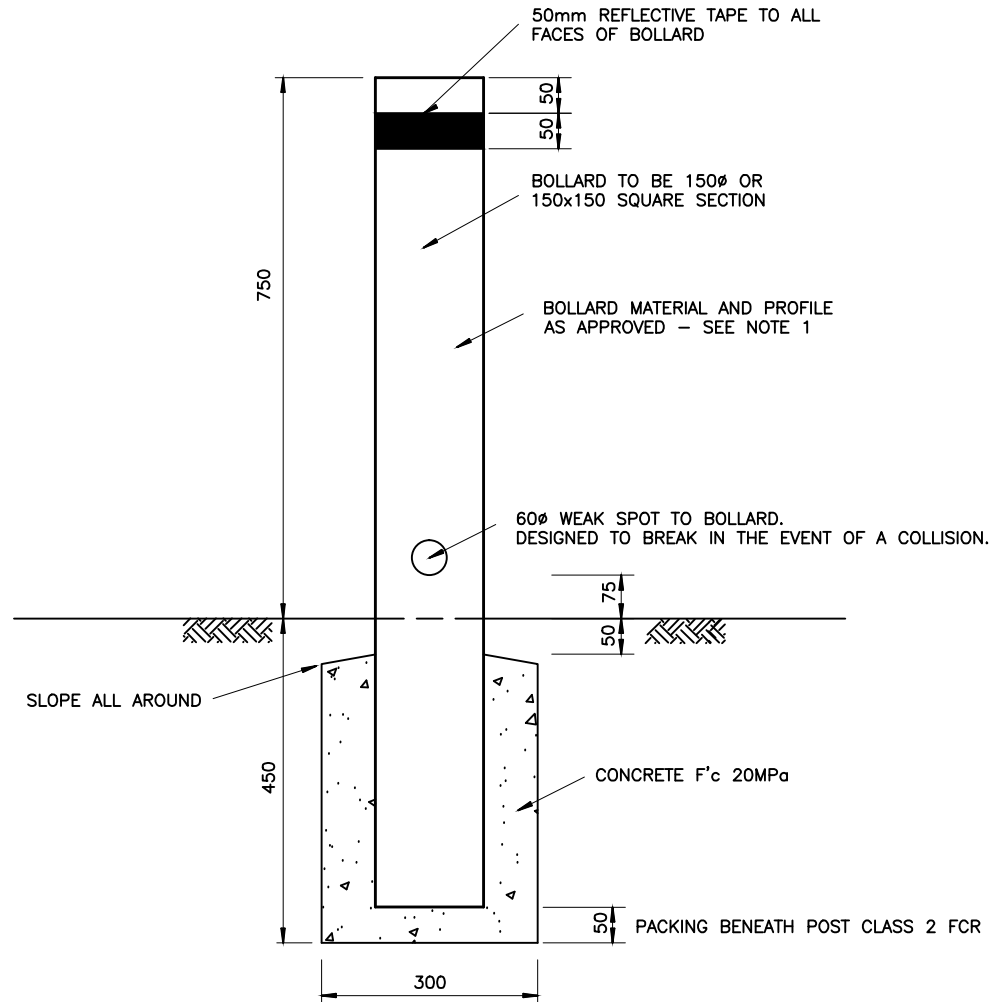
TYPICAL TIMBER BOLLARD SECTION
