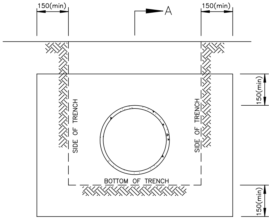
END VIEW
