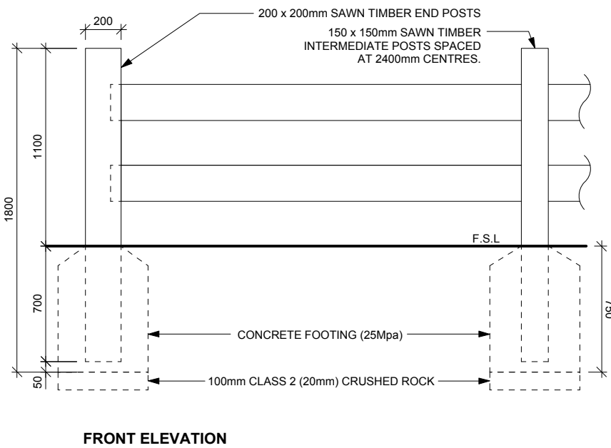
TYPICAL POST AND RAIL FENCE
