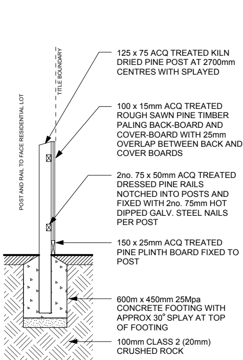
TYPICAL TIMBER PALING AND PICKET FENCE
